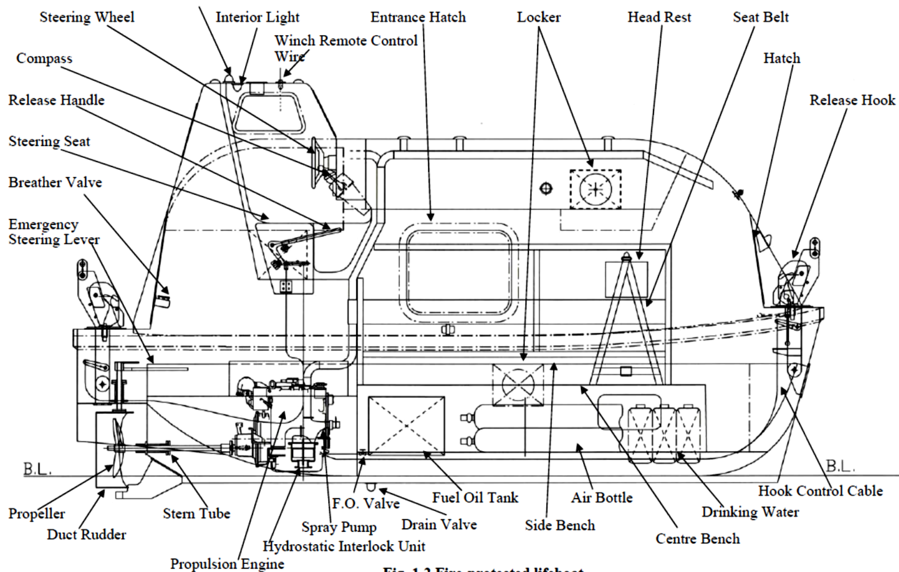
Fig. 1.2 Fire-protected lifeboat
